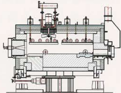
转底炉结构图 Structrue chart of Rotary Furnace
