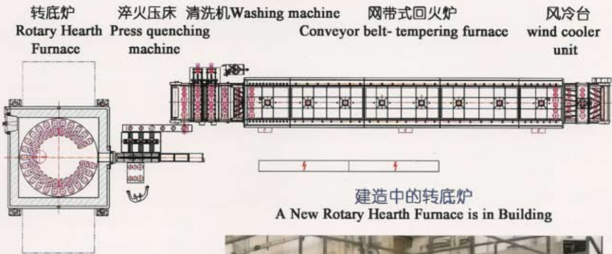
转底炉压淬回火生产线布置图 The Layout of Rotary Hearth Furnace Press Quenching Plants
